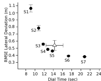
Figure 1: Model (dots) and human (triangle) data for total dialing time against lateral deviation
