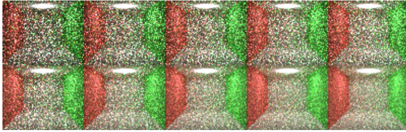
Fig. 4. Test scene 1 sampled using 100,200,300,400 and 500 samples pr. pixel. The top row shows the results using standard importance sampling and the bottom row shows the results when the information from the photon map is added
