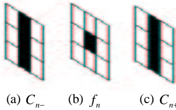
Figure 6: Window structure for spatial-temporal filtering in ROD for dirt detection.
