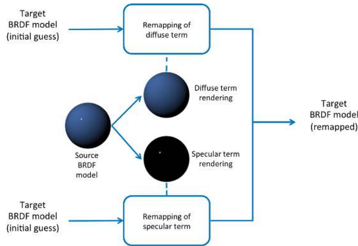
Figure 4. BRDF remapping scheme in two stages. Diffuse and specular components are remapped independently.
