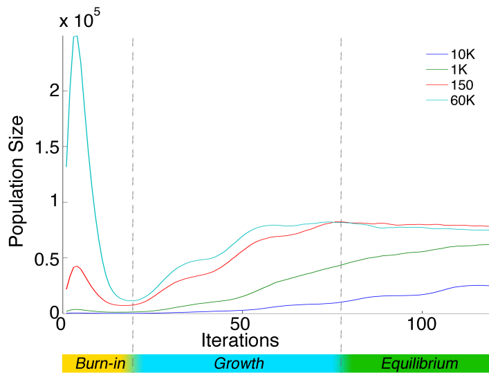
Figure 14. Comparison of the total population size over a 120 year simulation when using different numbers of initial trees (numbers in legend). Different phases of growth are highlighted with a gradient scale (as there is some variation between experiments).
