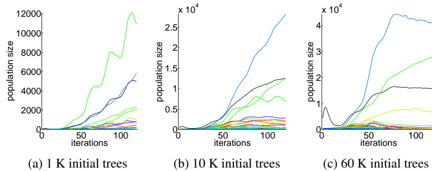
Figure 9. Analysis of the effect of initial number of trees over a 120-year simulation. Plots are shown of the total population (thick black lines scaled down for visualization) and the populations of each of the species.
