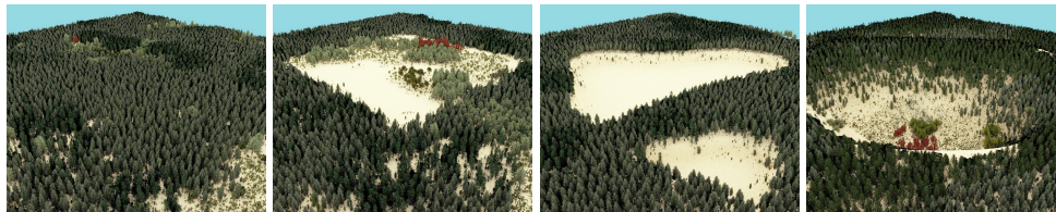
Figure 1. Our algorithm simulates realistic foliage cover for landscapes and allows for several modes of editability. From left: initial burn-in of the simulation; sparsifying a specified region; adding a lake to the landscape; simulating the same species on a different terrain.
