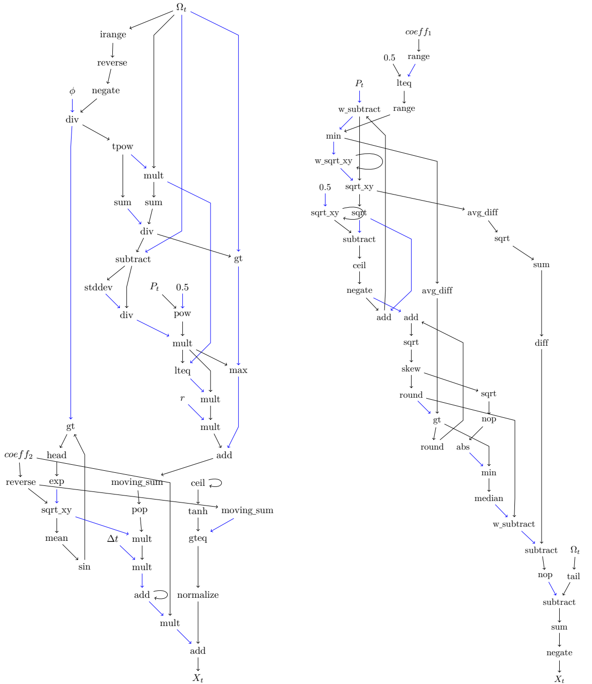
(a) An evolved version of ShoreFor incorporating an additional computational "module" near the output node
