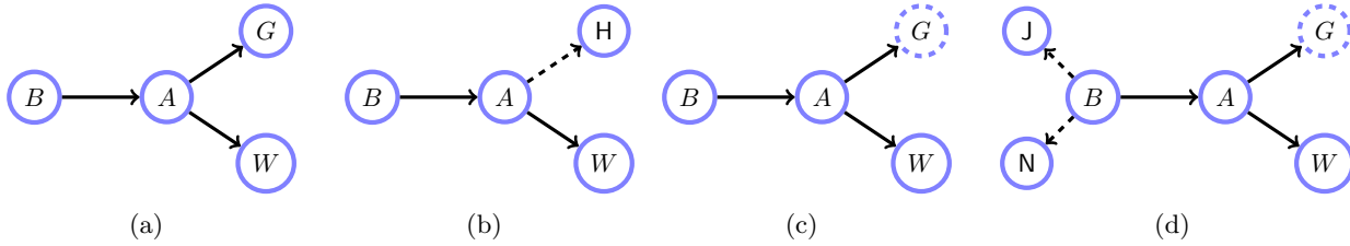
Figure 3.2: (a) : Mr Holmes' burglary worries as given in [222]: (B)urglar, (A)larm, (W)atson, Mrs (G)ibbon). (b) : Virtual Evidence can be represented by a dashed line. (c) : Modified problem. Mrs Gibbon is not drinking but somewhat deaf; we represent such uncertain (soft-evidence) by a circle. (d) : Holmes gets additional information from his neighbour Mrs (N)osy and informant Dodgy (J)oe.
