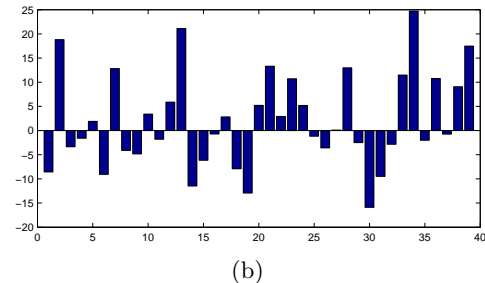
Figure 23.13: Using a linear chain CRF to learn the sequences in table(23.1). (a): The evolution of the log likelihood under gradient ascent. (b): The learned parameter vector \lambda at the end of training.
