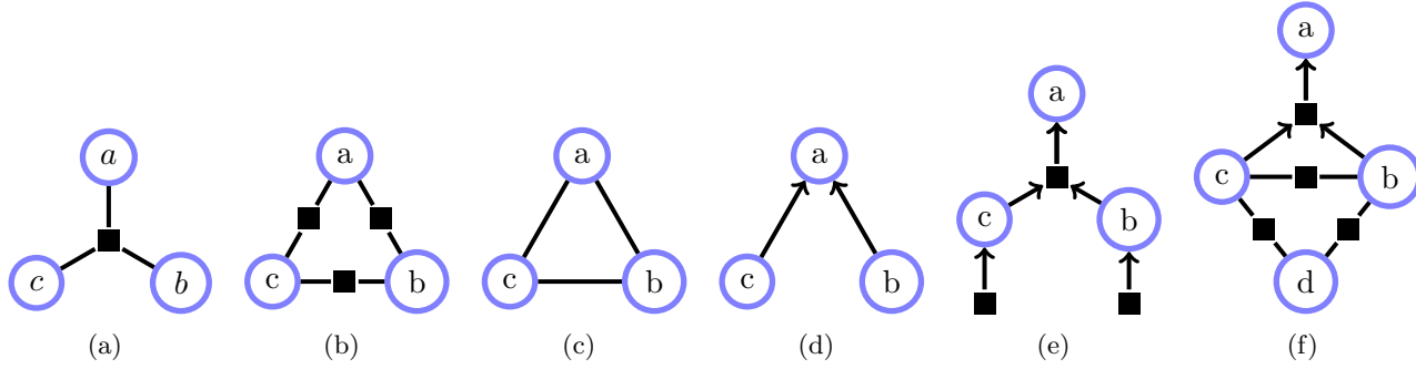
Figure 4.8: (a) : \phi(a, b, c) . (b) : \phi(a, b)\phi(b, c)\phi(c, a) . (c) : \phi(a, b, c) . Both (a) and (b) have the same undirected graphical model, (c). (e) : Directed FG of the BN in (d). (a) is an undirected FG of (d). The advantage of (e) over (a) is that information regarding the marginal independence of variables b and c is clear from graph (e), whereas one could only ascertain this by examination of the numerical entries of the factors in graph (a). (f) : A partially directed FG of p(a|b, c)\phi(d, c)\phi(b, d) . No directed, undirected or chain graph can represent both the conditional and marginal independence statements expressed by this graph and also the factored structure of the undirected terms.
