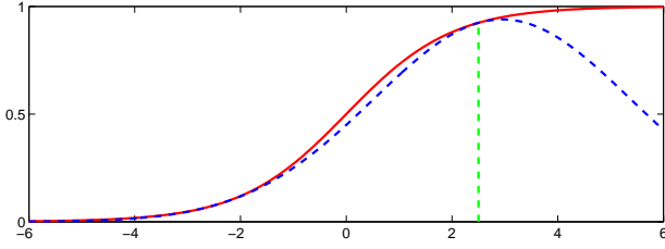
Figure 18.6: The logistic sigmoid \sigma(x) = 1/(1 + \exp(-x)) (red) and a Gaussian lower bound (blue dashed curve) with operating point 2.5.
