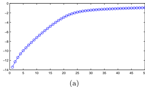
Figure 23.13: Using a linear chain CRF to learn the sequences in table(23.1). (a): The evolution of the log likelihood under gradient ascent. (b): The learned parameter vector \lambda at the end of training.
