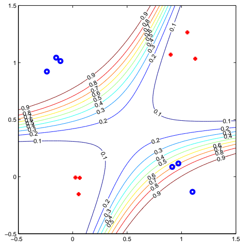
Figure 17.12: Logistic regression p(c = 1|\mathbf{x}) = \sigma(\mathbf{w}^\top \boldsymbol{\phi}(\mathbf{x})) using a quadratic function \boldsymbol{\phi}(\mathbf{x}) = (1, x_1, x_2, x_1^2, x_2^2, x_1x_2)^\top . 1000 iterations of gradient ascent training were performed with a learning rate \eta = 0.1 . Plotted are the datapoints for the two classes (red cross) and (blue circle) and the equal probability contours. The decision boundary is the 0.5-probability contour. See demoLogRegNonLinear.m .
