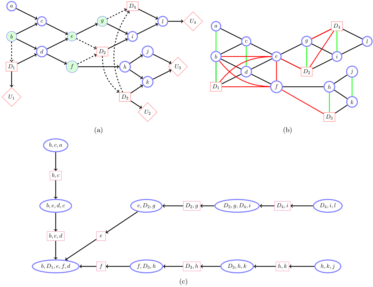
Figure 7.8: (a) : Influence Diagram, adapted from [148]. Causal consistency is satisfied since there is a directed path linking the all decisions in sequence. The partial ordering is b \prec D_1 \prec (e, f) \prec D_2 \prec (\cdot) \prec D_3 \prec g \prec D_4 \prec (a, c, d, h, i, j, k, l) . (b) : Moralised and strongly triangulated graph. Moralisation links are in green, strong triangulation links are in red. (c) : Strong Junction Tree. Absorption passes information from the leaves of the tree towards the root.
