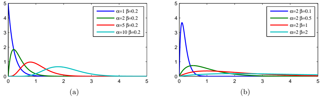
Figure 8.3: Gamma distribution. (a): varying \alpha for fixed \beta . (b): varying \beta for fixed \alpha .
