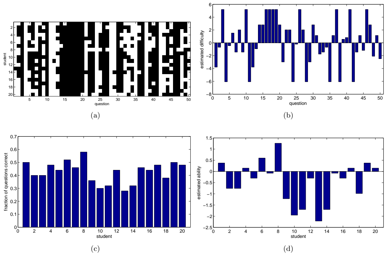
Figure 22.2: Rasch model. (a): The data of correct answers (white) and incorrect answers (black). (b): The estimated latent difficulty of each question. (c): The fraction of questions each student answered correctly. (d): The estimated latent ability.
