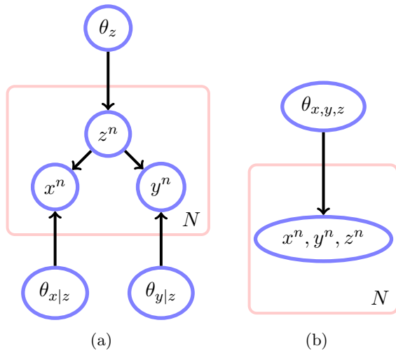
Figure 9.12: Bayesian conditional independence test using Dirichlet priors on the tables. (a): A model \mathcal{H}_{indep} for conditional independence x \perp\!\!\!\perp y | z . (b): A model \mathcal{H}_{dep} for conditional dependence x \not\perp\!\!\!\perp y | z . By computing the likelihood of the data under each model, a numerical score for the validity of the conditional independence assumption can be formed. See demoCondindepEmp.m .
