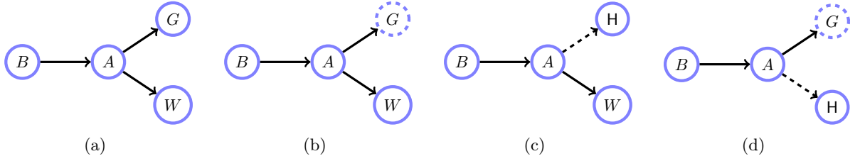
Figure 3.3: (a): Mr Holmes' burglary worries as given in [237]: (B)urglar, (A)larm, (W)atson, Mrs (G)ibbon. (b): Mrs Gibbon's uncertain evidence represented by a dashed circle. (c): Virtual evidence or the replacement of unreliable evidence can be represented by a dashed line. (d): Mrs Gibbon is uncertain in her evidence. Holmes also replaces the unreliable Watson with his own interpretation.
