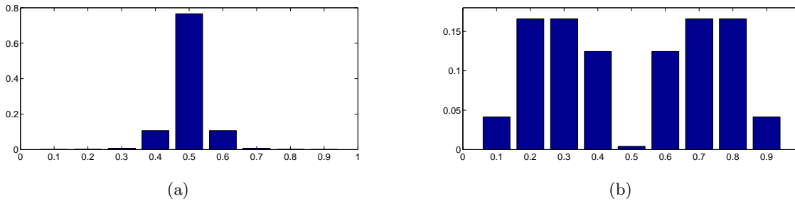
Figure 12.1: (a) : Discrete prior p(\theta|M_{fair}) model of a ‘fair’ coin. A perfectly unbiased coin has \theta = 0.5 , which would corresponds to a prior \delta(\theta, 0.5) – however, we assume a more general form here to illustrate how richer prior assumptions can be used. (b) : Prior p(\theta|M_{biased}) for a biased ‘unfair’ coin. In both cases we are making explicit choices here about what we consider to be a ‘fair’ and ‘unfair’.
