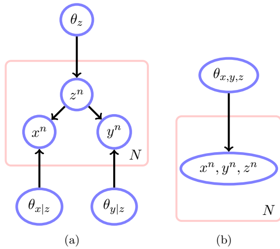
Figure 9.12: Bayesian conditional independence test using Dirichlet priors on the tables. (a): A model \mathcal{H}_{indep} for conditional independence x \perp y | z . (b): A model \mathcal{H}_{dep} for conditional dependence x \not\perp y | z . By computing the likelihood of the data under each model, a numerical score for the validity of the conditional independence assumption can be formed. See demoCondindepEmp.m .
