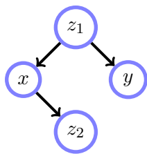
Figure 9.13: Conditional independence test of x \perp\!\!\!\perp y \mid z_1, z_2 with x, y, z_1, z_2 having 3, 2, 4, 2 states respectively. From the oracle belief network shown, in each experiment the tables are drawn at random and 20 examples are sampled to form a dataset. For each dataset a test is carried out to determine if x and y are independent conditioned on z_1, z_2 (the correct answer being that they are independent). Over 500 experiments, the Bayesian conditional independence test correctly states that the variables are conditionally independent 74% of the time, compared with only 50% accuracy using the chi-square mutual information test. See demoCondindepEmp.m .
