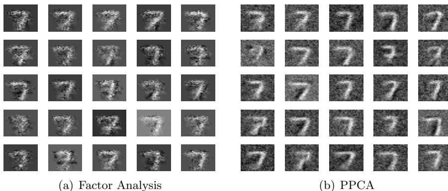
Figure 21.8: (a): 25 samples from the learned FA model. Note how the noise variance depends on the pixel, being zero for pixels on the boundary of the image. (b): 25 samples from the learned PPCA model with the same noise variance on each pixel.
