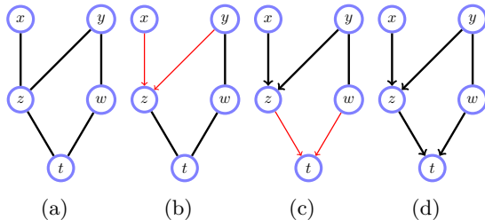
Figure 9.11: Skeleton orientation algorithm. (a) : The skeleton along with S_{x,y} = \emptyset, S_{x,w} = \emptyset, S_{z,w} = y, S_{x,t} = \{z, w\}, S_{y,t} = \{z, w\} . (b) : z \notin S_{x,y} , so form collider. (c) : t \notin S_{z,w} , so form collider. (d) : Final partially oriented DAG. The remaining edge may be oriented as desired, without violating the DAG condition. See also demoPCoracle.m .
