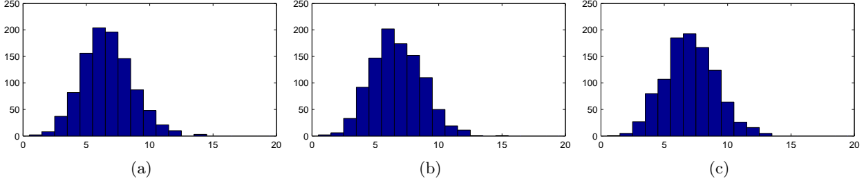
Figure 20.13: The distribution of the number of unique clusters U when indicators are sampled from a Polya distribution equation (20.5.8), with \alpha = 2 , and N = 50 datapoints. (a) : K = 50 , (b) : K = 100 , (c) : K = 1000 . Even though the number of available clusters K is larger than the number of datapoints, the number of used clusters U remains constrained. See demoPolya.m .
