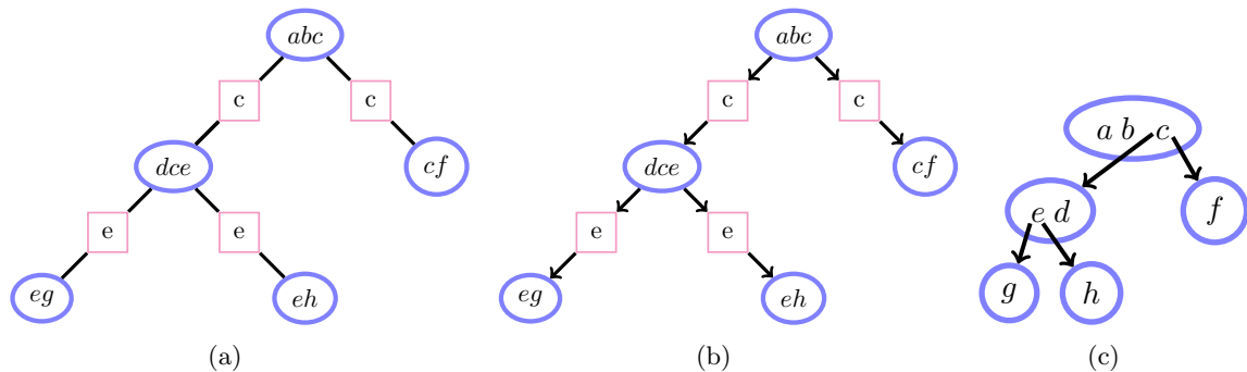
Figure 6.13: (a): Junction tree. (b): Directed junction tree in which all edges are consistently oriented away from the clique ( abc ). (c): A set chain formed from the junction tree by reabsorbing each separator into its child clique.
