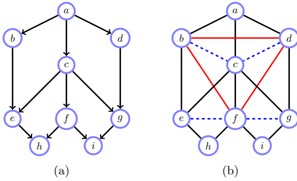
Figure 6.11: (a): Original loopy Belief Network. (b): The moralisation links (dashed) are between nodes e and f and between nodes f and g . The other additional links come from triangulation. The clique size of the resulting clique tree (not shown) is four.
