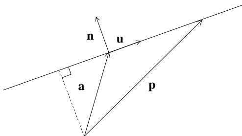
Figure 29.2: A line can be specified by some position vector on the line, \mathbf{a} , and a unit vector along the direction of the line, \mathbf{u} . In 2 dimensions, there is a unique direction, \mathbf{n} , perpendicular to the line. In three dimensions, the vectors perpendicular to the direction of the line lie in a plane, whose normal vector is in the direction of the line, \mathbf{u} .
