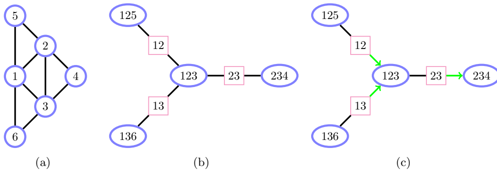
Figure 6.11: (a) : Markov network. (b) : Junction tree. Under absorption, once we have absorbed from 125 to 123 and 136 to 123, the result of these absorptions is stored in the new potential on 123. After this we can absorb from 123 to 234 by operating on the 123 potential and then sending this information to 234. (c) : In Shafer-Shenoy updating, we send a message from a clique to a neighbouring clique based on the product of all incoming messages.
