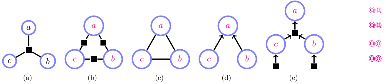
Figure 4.8: (a): \phi(a, b, c) . (b): \phi(a, b)\phi(b, c)\phi(c, a) . (c): \phi(a, b, c) . Both (a) and (b) have the same undirected graphical model, (c). (d): (a) is an undirected FG of (d). (e): Directed FG of the BN in (d). A directed factor represents a term p(\text{children}|\text{parents}) . The advantage of (e) over (a) is that information regarding the marginal independence of variables b and c is clear from graph (e), whereas one could only ascertain this by examination of the numerical entries of the factors in graph (a).
