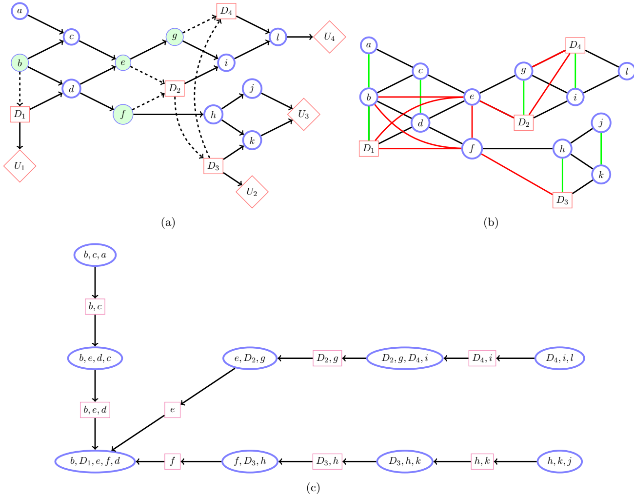
Figure 7.7: (a): Influence Diagram, adapted from [? ]. Causal consistency is satisfied since there is a directed path linking all decisions in sequence. The partial ordering is b \prec D_1 \prec (e, f) \prec D_2 \prec (\cdot) \prec D_3 \prec g \prec D_4 \prec (a, c, d, h, i, j, k, l) . (b): Moralised and strongly triangulated graph. Moralisation links are in green, strong triangulation links are in red. (c): Strong Junction Tree. Absorption passes information from the leaves of the tree towards the root.
