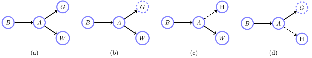
Figure 3.3: (a): Mr Holmes' burglary worries as given in [? ]: (B)urglar, (A)larm, (W)atson, Mrs (G)ibbon. (b): Mrs Gibbon's uncertain evidence represented by a dashed circle. (c): Virtual evidence or the replacement of unreliable evidence can be represented by a dashed line. (d): Mrs Gibbon is uncertain in her evidence. Holmes also replaces the unreliable Watson with his own interpretation.
