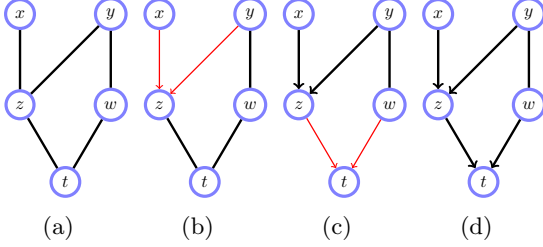
Figure 9.11: Skeleton orientation algorithm. (a): The skeleton along with S_{x,y} = \emptyset, S_{x,w} = \emptyset, S_{z,w} = y, S_{x,t} = \{z, w\}, S_{y,t} = \{z, w\} . (b): z \notin S_{x,y} , so form collider. (c): t \notin S_{z,w} , so form collider. (d): Final partially oriented DAG. The remaining edge may be oriented as desired, without violating the DAG condition. See also demoPCoracle.m .
