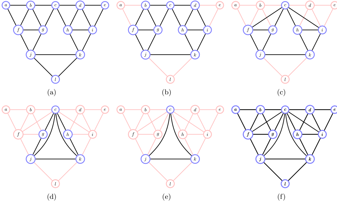
Figure 6.8: (a) : Markov network for which we seek a triangulation via greedy variable elimination. We first eliminate the simplicial nodes a, e, l . (b) : We then eliminate variables b, d since these only add a single extra link to the induced graph. (c) : There are no simplicial nodes at this stage, and we choose to eliminate f and i , each elimination adding only a single link. (d) : We eliminate g and h since these are simplicial. (e) : The remaining variables \{c, j, k\} may be eliminated in any order. (f) : Final triangulation. The variable elimination (partial) order is \{a, e, l\}, \{b, d\}, \{f, i\}, \{g, h\}, \{c, j, k\} where the brackets indicate that the order in which the variables inside the bracket are eliminated is irrelevant. Compared with the triangulation produced by the max-cardinality checking approach in fig(6.10d), this triangulation is more parsimonious.
