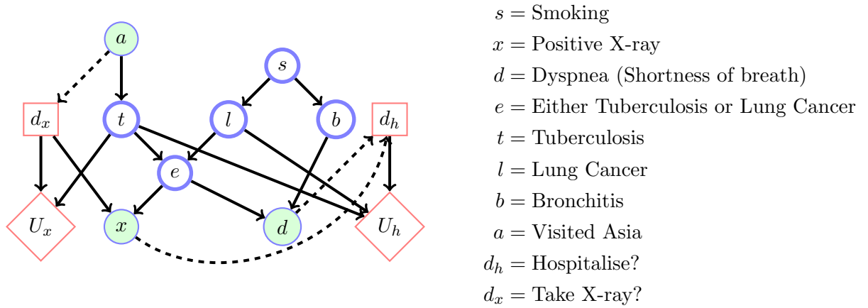
Figure 7.14: Influence Diagram for the ‘Chest Clinic’ Decision example.
