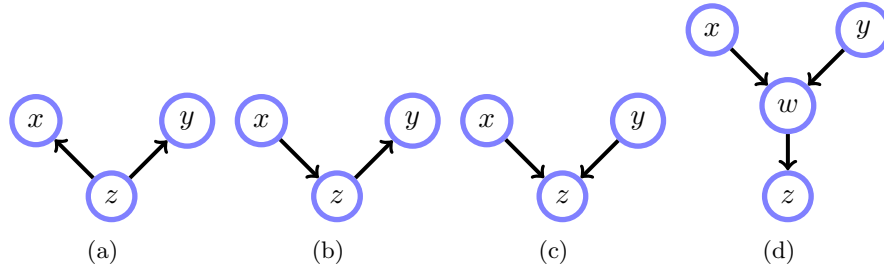
Figure 3.7: In graphs (a) and (b), variable z is not a collider. (c): Variable z is a collider. Graphs (a) and (b) represent conditional independence x \perp\!\!\!\perp y \mid z . In graphs (c) and (d), x and y are ‘graphically’ conditionally dependent given variable z .
