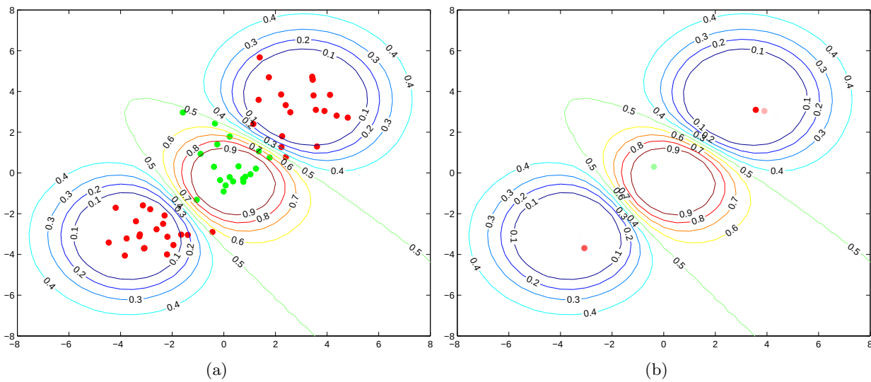
Figure 18.8: Classification using the RVM with RBF e^{-\lambda(\mathbf{x}-\mathbf{m})^2} , placing a basis function on a subset of the training data points. The green points are training data from class 1, and the red points are training data from class 0. The contours represent the probability of being in class 1. (a) : Training points. (b) : The training points weighted by their relevance value 1/\alpha_n . Nearly all the points have a value so small that they effectively vanish. See demoBayesLogRegRVM.m
