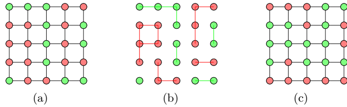
Figure 27.10: Swendsson-Wang updating for p(x) \propto \prod_{i \sim j} \exp \beta \mathbb{I}[x_i = x_j] . (a) : Current sample of states (here on a nearest neighbour lattice). (b) : Like coloured neighbours are bonded together with probability 1 - e^{-\beta} , forming clusters of variables. (c) : Each cluster is given a random colour, forming the new sample.
