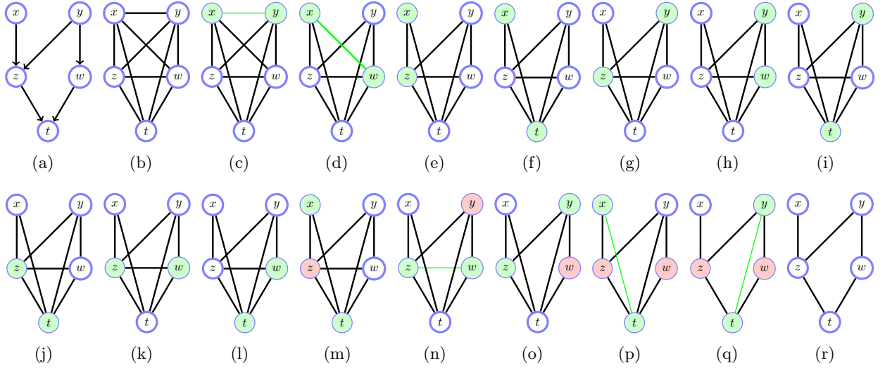
Figure 9.10: PC algorithm. (a) : The BN from which data is assumed generated and against which conditional independence tests will be performed. (b) : The initial skeleton is fully connected. (c-l) : In the first round ( i = 0 ) all the pairwise mutual informations x \perp\!\!\!\perp y | \emptyset are checked, and the link between x and y removed if deemed independent (green line). (m-o) : i = 1 . We now look at connected subsets on three variables x, y, z of the remaining graph, removing the link x - y if x \perp\!\!\!\perp y | z is true. Not all steps are shown. (p,q) : i = 2 . We now examine all x \perp\!\!\!\perp y | \{a, b\} . The algorithm terminates after this round (when i gets incremented to 3) since there are no nodes with 3 or more neighbours. (r) : Final skeleton. During this process the sets S_{x,y} = \emptyset, S_{x,w} = \emptyset, S_{z,w} = y, S_{x,t} = \{z, w\}, S_{y,t} = \{z, w\} were found. See also demoPCoracle.m
