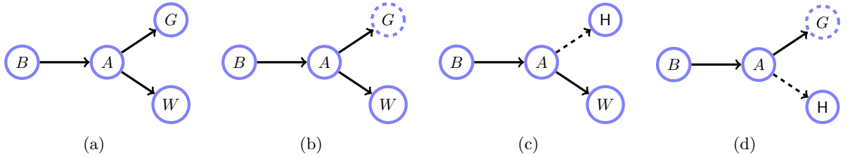
Figure 3.3: (a) : Mr Holmes’ burglary worries as given in [217]: (B)urglar, (A)larm, (W)atson, Mrs (G)ibbon. (b) : Mrs Gibbon’s uncertain evidence represented by a dashed circle. (c) : Virtual evidence or the replacement of unreliable evidence can be represented by a dashed line. (d) : Mrs Gibbon is uncertain in her evidence. Holmes also replaces the unreliable Watson with his own interpretation.
