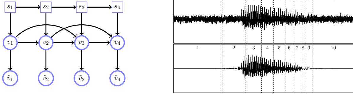
Figure 24.9: (a) : A latent switching (second order) AR model. Here the s_t indicates which of a set of 10 available AR models is active at time t . The square nodes emphasise that these are discrete variables. The ‘clean’ AR signal v_t , which is not observed, is corrupted by additive noise to form the noisy observations \tilde{v}_t . In terms of inference, conditioned on \tilde{v}_{1:T} , this can be expressed as a Switching LDS, chapter(25). (b) : Signal reconstruction using the latent switching AR model in (a). Top: noisy signal \tilde{v}_{1:T} ; bottom: reconstructed clean signal v_{1:T} . The dashed lines and the numbers show the most-likely state segmentation \arg \max_{s_{1:T}} p(s_{1:T}|\tilde{v}_{1:T}) .
