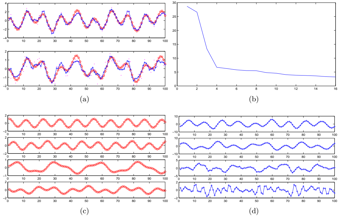
Figure 24.5: Learning the parameters of a noisy LDS with V = 2 , H = 4 . (a) : The small points are the visible data, circles the noise free visible observations, and the crosses the estimates of the noise free observations based on using the subspace method. (b) : Singular values. In a noise free case, only H = 4 singular values will be non-zero. The noise in this problem means that additional singular values appear. (c) : Hidden values used to generate the data. (d) : Hidden values estimated by the subspace method, formed from the principal 4-dimensional subspace.
