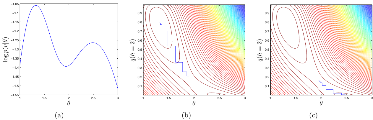
Figure 11.2: (a) : The log likelihood for the model described in example(51). (b) : Contours of the lower bound LB(q(h = 2), \theta) . For an initial choice q(h = 2) = 0.5 and \theta = 1.9 , successive updates of the E (vertical) and M (horizontal) steps are plotted. (c) : Starting at \theta = 1.95 , the EM algorithm converges to a local optimum.
