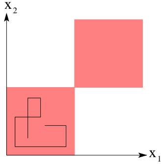
Figure 27.6: A two dimensional distribution for which Gibbs sampling fails. The distribution has mass only in the shaded quadrants. Gibbs sampling proceeds from the l^{th} sample state (x_1^l, x_2^l) and then sampling from p(x_2|x_1^l) , which we write (x_1^{l+1}, x_2^{l+1}) where x_1^{l+1} = x_1^l . One then continues with a sample from p(x_1|x_2 = x_2^{l+1}) , etc. If we start in the lower left quadrant and proceed this way, the upper right region is never explored. This is a case where the sampler is non-ergodic.
