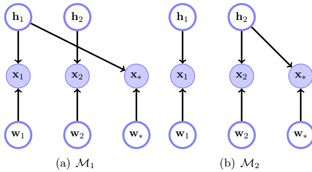
Figure 21.6: Face recognition model (depicted only for a single exemplar per person, J = 1 ). (a) : In model \mathcal{M}_1 the test image (or ‘probe’) \mathbf{x}_* is assumed to be from person 1, albeit with a different pose/illumination. (b) : For model \mathcal{M}_2 the test image is assumed to be from person 2. One calculates p(\mathbf{x}_1, \mathbf{x}_2, \mathbf{x}_* | \mathcal{M}_1) and p(\mathbf{x}_1, \mathbf{x}_2, \mathbf{x}_* | \mathcal{M}_2) and then uses Bayes’ rule to infer which person the test image \mathbf{x}_* most likely belongs.
