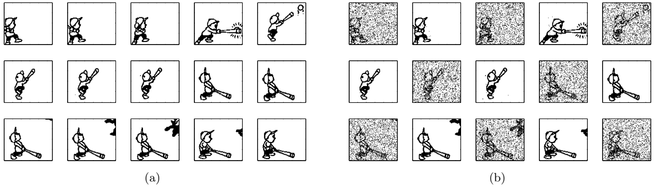
Figure 26.4: (a): Original T = 25 binary video sequence on a set of 81 \times 111 = 8991 neurons. (b): The reconstructions beginning from a 20% noise perturbed initial state. Every odd time reconstruction is also randomly perturbed. Despite the high level of noise the basis of attraction of the pattern sequence is very broad and the patterns immediately fall back close to the pattern sequence even after a single timestep.
