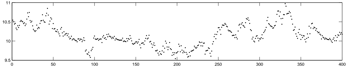
Figure 25.8: Data from an intermittent mean-reverting process. See exercise(238).
