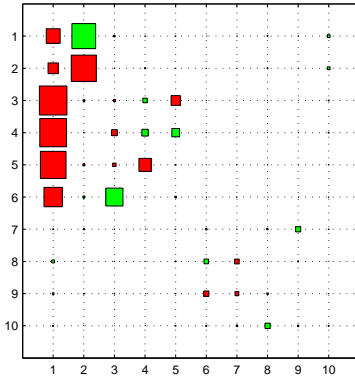
Figure 15.9: Hinton Diagram of the eigenvector matrix \mathbf{E} where each eigenvector column is scaled by the corresponding eigenvalue. Red indicates positive and green negative (the area of each square corresponds to the magnitude), showing that there are only a few large eigenvalues. Note that the overall sign of any eigenvector is irrelevant. The first eigenvector corresponds to a topic in which the words influenza , flu , headache , nose , temperature , bed are prevalent. The second eigenvector denotes that there is negative correlation between the occurrence of influenza and flu .
