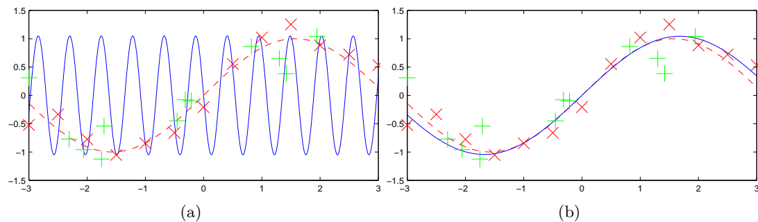
Figure 13.5: (a) : The unregularised fit ( \lambda = 0 ) to training given by \times . Whilst the training data is well fitted, the error on the validation examples, + is high. (b) : The regularised fit ( \lambda = 0.5 ). Whilst the train error is high, the validation error (which is all important) is low. The true function which generated this noisy data is the dashed line; the function learned from the data is given by the solid line.
