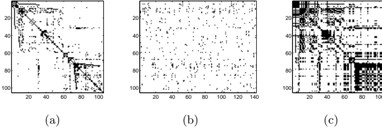
Figure 20.21: (a) : Adjacency matrix of 105 Political Books (black=1). (b) : Clique matrix: 521 non-zero entries. (c) : Adjacency reconstruction using an Approximate Clique Matrix with 10 cliques – see also fig(20.22) and demoCliqueDecomp.m .
