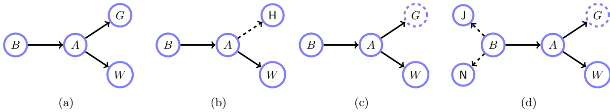
Figure 3.3: (a) : Mr Holmes' burglary worries as given in [213]: (B)urglar, (A)larm, (W)atson, Mrs (Gibbon). (b) : Virtual Evidence can be represented by a dashed line. (c) : Modified problem. Mrs Gibbon is not drinking but somewhat deaf; we represent such uncertain (soft-evidence) by a circle. (d) : Holmes gets additional information from his neighbour Mrs (N)osy and informant Dodgy (J)oe.
