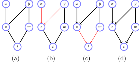
Figure 9.10: Skeleton orientation algorithm. (a) : The skeleton along with S_{x,y} = \emptyset, S_{x,w} = \emptyset, S_{z,w} = y, S_{x,t} = \{z, w\}, S_{y,t} = \{z, w\} . (b) : z \notin S_{x,y} , so form collider. (c) : t \notin S_{z,w} , so form collider. (d) : Final partially oriented DAG. The remaining edge may be oriented as desired, without violating the DAG condition. See also demoPCoracle.m .
