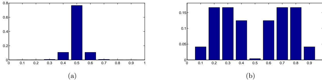
Figure 12.1: (a) : Discrete prior model of a ‘fair’ coin. (b) : Prior for a biased ‘unfair’ coin. In both cases we are making explicit choices here about what we consider to be a ‘fair’ and an ‘unfair’.
