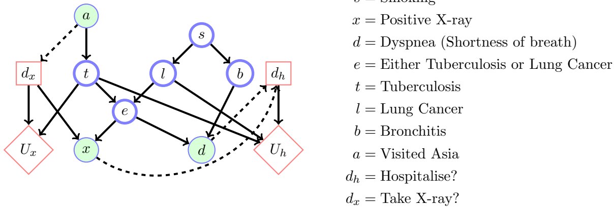
Figure 7.13: Influence Diagram for the ‘Chest Clinic’ Decision example.
