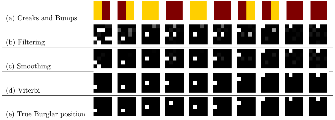
Figure 23.7: Localising the burglar through time for 10 time steps. (a) : Each panel represents the visible information v_t = (v_t^{creak}, v_t^{bump}) , where v_t^{creak} = 1 means that there was a ‘creak in the floorboard’ ( v_t^{creak} = 2 otherwise) and v_t^{bump} = 1 meaning ‘bumped into something’ (and is in state 2 otherwise). There are 10 panels, one for each time t = 1, \dots, 10 . The left half of the panel represents v_t^1 and the right half v_t^2 . The lighter colour represents the occurrence of a creak or bump, the darker colour the absence. (b) : The filtered distribution p(h_t|v_{1:t}) representing where we think the burglar is. (c) : The smoothed distribution p(h_t|v_{1:10}) so that we can figure out where we think the burglar went. (d) : The most likely (Viterbi) burglar path \arg \max_{h_{1:10}} p(h_{1:10}|v_{1:10}) . (e) : The actual path of the burglar.
