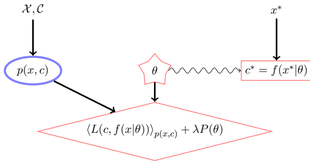
Figure 13.2: Empirical risk approach. Given the dataset \mathcal{X}, \mathcal{C} , a model of the data p(x, c) is made, usually using the empirical distribution. For a classifier f(x|\theta) , the parameter \theta is learned by minimising the penalised empirical risk with respect to \theta . The penalty parameter \lambda is set by validation. A novel input x^* is then assigned to class f(x^*|\theta) , given this optimal \theta .
