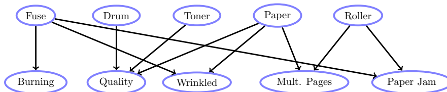
Figure 9.21: Printer Nightmare belief network. All variables are binary. The upper variables without parents are possible problems (diagnoses), and the lower variables consequences of problems (faults).
