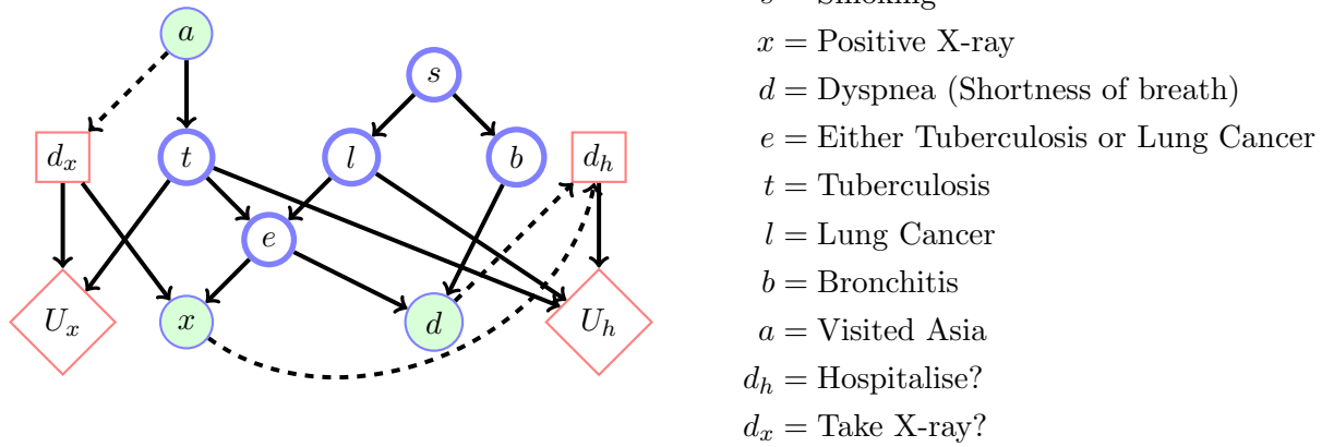
Figure 7.14: Influence Diagram for the ‘Chest Clinic’ Decision example.
