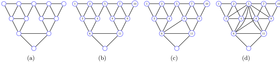
Figure 6.10: Starting with the Markov network in (a), the maximum cardinality check algorithm proceeds until (b), where an additional link is required, see (c). One continues until the fully triangulated graph (d) is found.
