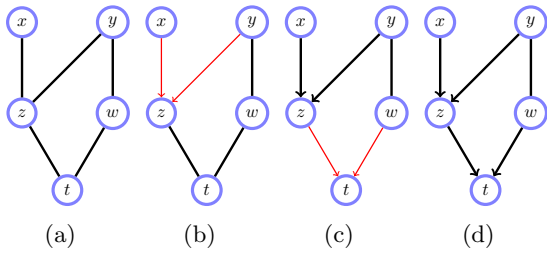
Figure 9.11: Skeleton orientation algorithm. (a): The skeleton along with S_{x,y} = \emptyset, S_{x,w} = \emptyset, S_{z,w} = y, S_{x,t} = \{z, w\}, S_{y,t} = \{z, w\} . (b): z \notin S_{x,y} , so form collider. (c): t \notin S_{z,w} , so form collider. (d): Final partially oriented DAG. The remaining edge may be oriented as desired, without violating the DAG condition. See also demoPCoracle.m .
